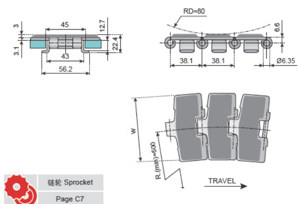
SS881TAB-G 防滑侧弯平顶链 SS881TAB-G WITH RUBBER TOP
