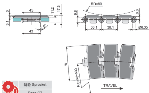
SS881G 防滑侧弯平顶链 SS881G WITH RUBBER TOP
